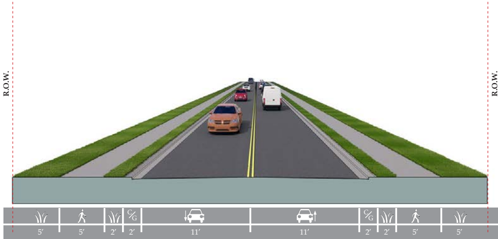
Example of 50-ft Local Street R.O.W.
